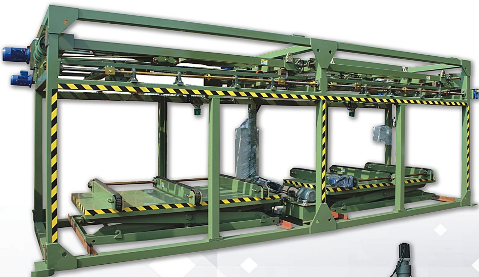
• Automatic Plywood Stacker
